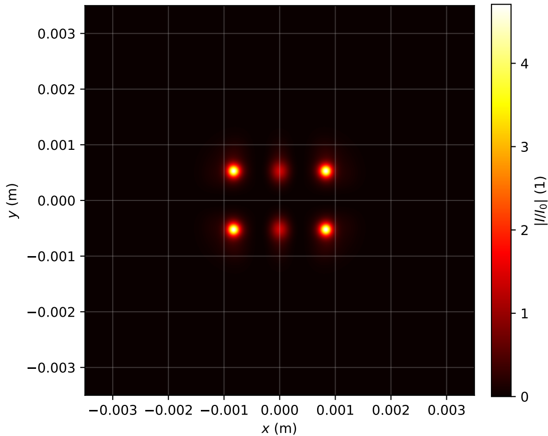
Intensity profile I(x, y, z = 0.478)/I_0 , \text{Pin}=7.0\text{Pcr} , artificial time
